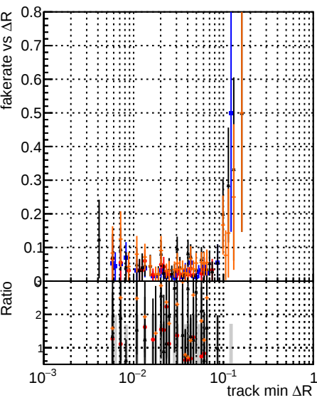
Fake rate vs \Delta R(\text{track, jet}) DQM original4 DQM resM4Fit initialStepReso DQM resM4Fit initialStepReso DQM resM4Fit initialStepReso wRejection25
