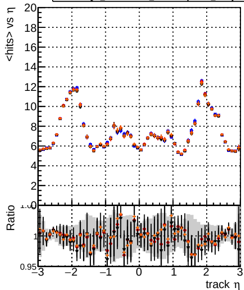
mean hits — DQM_original4 — DQM_testMkFitFit_initialStepReso — DQM_testMkFitFit_initialStepReso — DQM_testMkFitFit_initialStepReso_wRejection25
