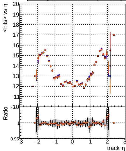
mean hits DQM_testMkFit_initialStepReso DQM_testMkFitFit_initialStepReso DQM_testMkFitFit_initialStepReso_wRejection25
