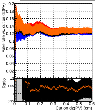
—●— DQM_testMkFitFit_initialStepReso —●— DQM_testMkFitFit_initialStepReso_wRejection25
