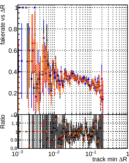
Fake rate vs \Delta R(\text{track, jet}) DOM original4 DOM testIMKFit initialStepReso DOM testIMKFit initialStepReso wRejection25
