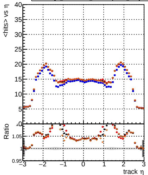
mean hit DQM_origina14 DQM_testMkFit_initialStepReso DQM_testMkFitFit_initialStepReso DQM_testMkFitFit_initialStepReso_wRejection25
