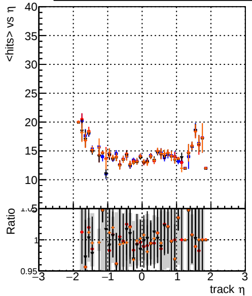
mean hits vs \eta DQM_original4 DQM_testMkFit_initialStepReso DQM_testMkFitFit_initialStepReso DQM_testMkFitFit_initialStepReso_wRejection25
