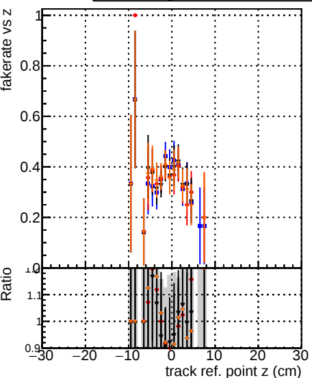
Fake rate vs v DOM original4 DOM testIMKFit_initialStepReso DOM testIMKFit_initialStepReso_wRejection25
