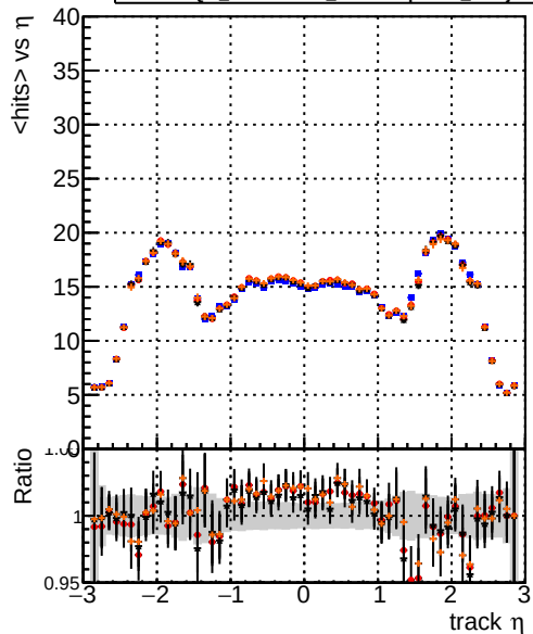
DQM_testMkFitFit_initialStepReso DQM_testMkFitFit_initialStepReso DQM_testMkFitFit_initialStepReso_wRejection25 DQM_testMkFitFit_initialStepReso mean hits
