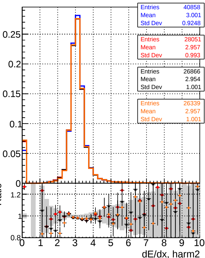
—●— DQM_original4 —●— DQM_testMkFit_initialStepReso —●— DQM_testMkFitFit_initialStepReso —●— DQM_testMkFitFit_initialStepReso_wRejection25
