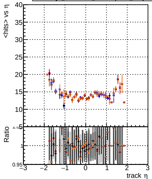
DQM_original4 DQM_testMkFit_fit_initialStepReso DQM_testMkFitFit_initialStepReso DQM_testMkFitFit_initialStepReso_wRejection25 mean hits
