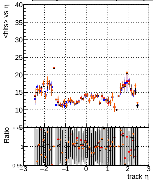
DQM_original4 DQM_testMkFit_initialStepReso DQM_testMkFitFit_initialStepReso DQM_testMkFitFit_initialStepReso_wRejection25 mean hits
