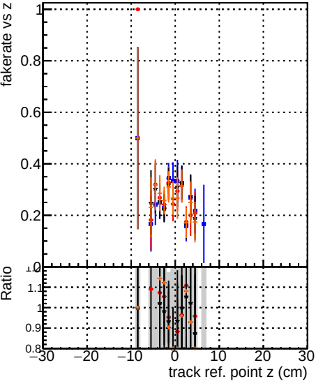
DOM original4 DOM testMKFit initialStepReso DOM testMKFit initialStepReso wRejection25
