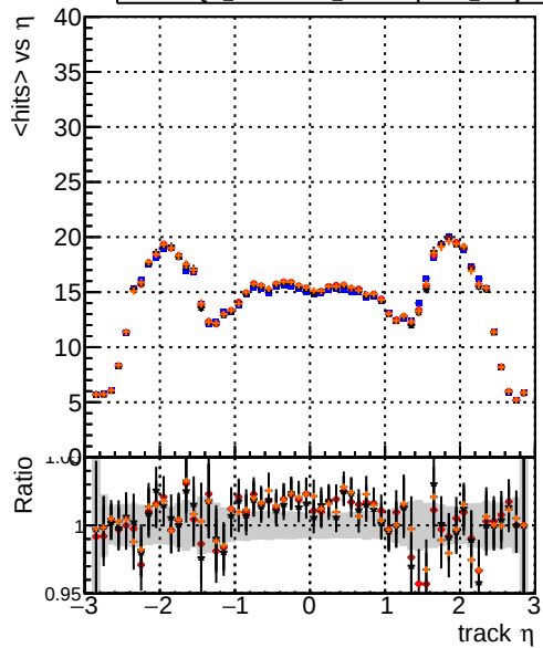
DQM_origMkFit4 DQM_testMkFit_initialStepReso DQM_testMkFitFit_initialStepReso DQM_testMkFitFit_initialStepReso_wRejection25 mean hit
