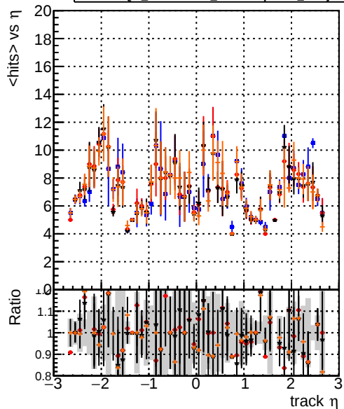
— DQM_testMkFit_initialStepReso — DQM_testMkFitFit_initialStepReso — DQM_testMkFitFit_initialStepReso_wRejection25 mean hit
