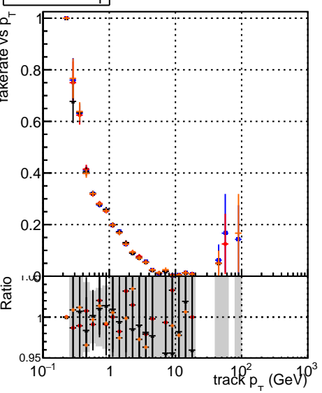
Fake rate vs p_T
