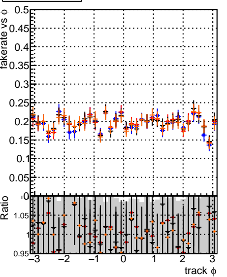
Fake rate vs \phi
