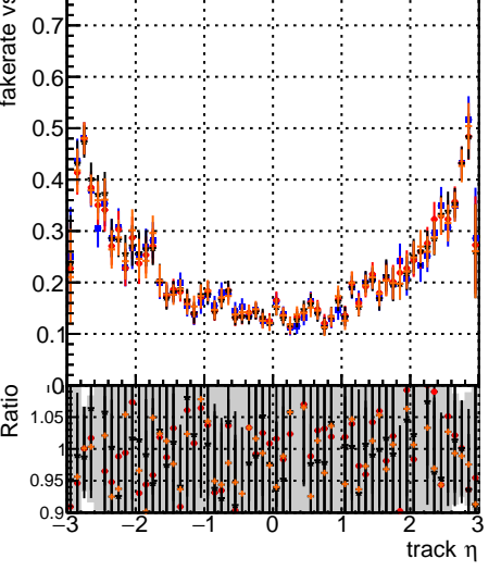
Fake rate vs \eta
