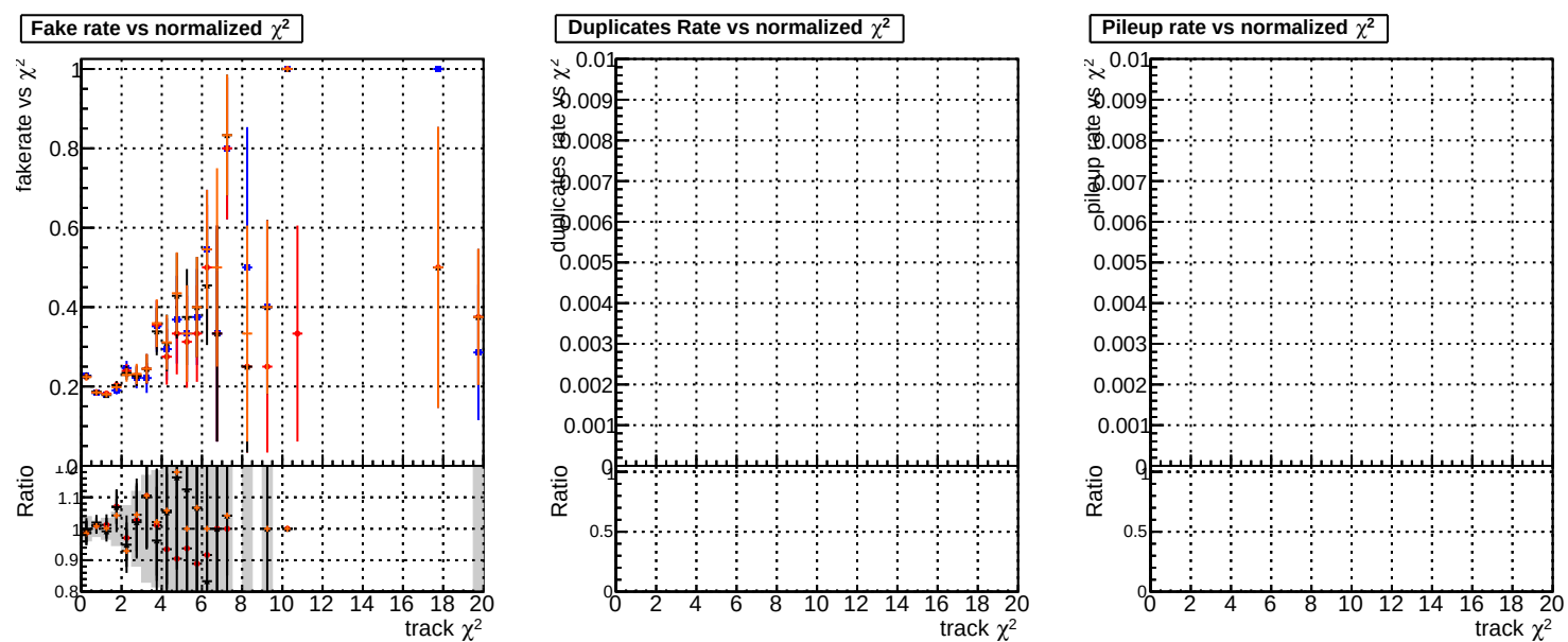
Fake rate vs. BQM original BQM test BQM test MRFF BQM test MRFF InitialStepReso BQM test MRFF InitialStepReso wRejection25
