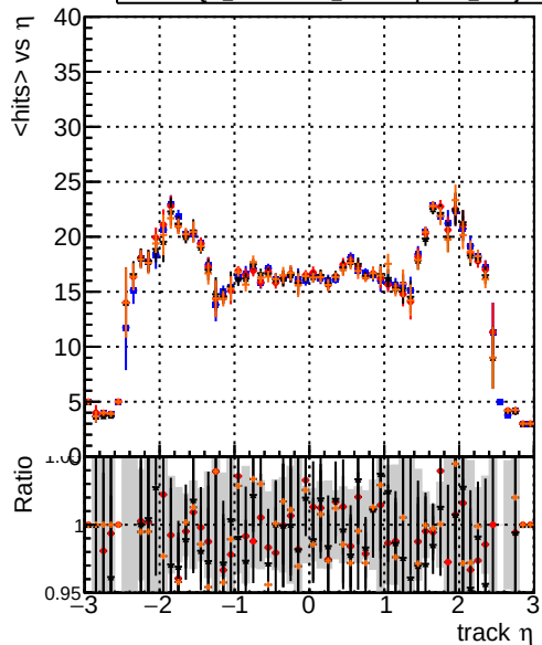
mean hits vs \eta DQM_original4 DQM_testMkFitFit_initialStepReso DQM_testMkFitFit_initialStepReso DQM_testMkFitFit_initialStepReso_wRejection25
