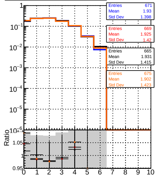
— DQM_original4 — DQM_testMkFit_initialStepReso — DQM_testMkFitFit_initialStepReso — DQM_testMkFitFit_initialStepReso_wRejection25 mean hit
