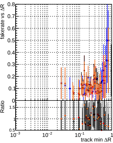
Fake rate vs ΔR(track, jet) DOM original DOM test DOM fit DOM test fit wRejection25
