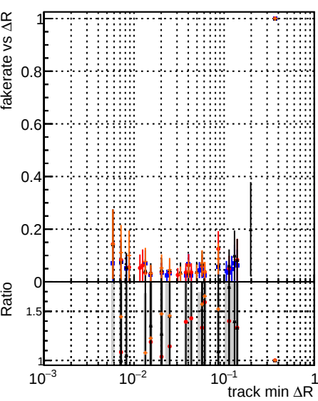
Fake rate vs ΔR(track, jet) DOM original4 DOM testIMKFit_initialStepReso DOM testIMKFit_initialStepReso_wRejection25 DOM testIMKFit_initialStepReso
