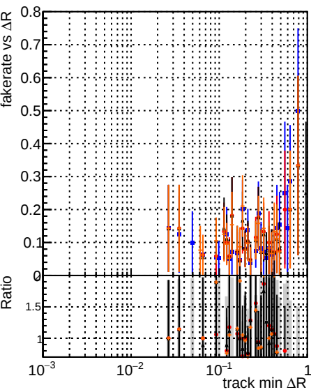
Fake rate vs ΔR(track, jet) DOM original DOM test DOM MC Fit initialStepReso DOM MC Fit initialStepReso wRejection25
