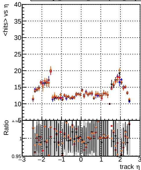
DQM_original4 DQM_testMkFit_initialStepReso DQM_testMkFitFit_initialStepReso DQM_testMkFitFit_initialStepReso_wRejection25
