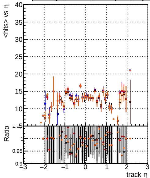
mean hit DQM_original4 DQM_testMkFit_initialStepReso DQM_testMkFitFit_initialStepReso DQM_testMkFitFit_initialStepReso_wRejection25
