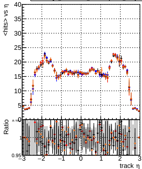
— DQM_original4 — DQM_testMkFit_initialStepReso — DQM_testMkFitFit_initialStepReso — DQM_testMkFitFit_initialStepReso_wRejection25 mean hit
