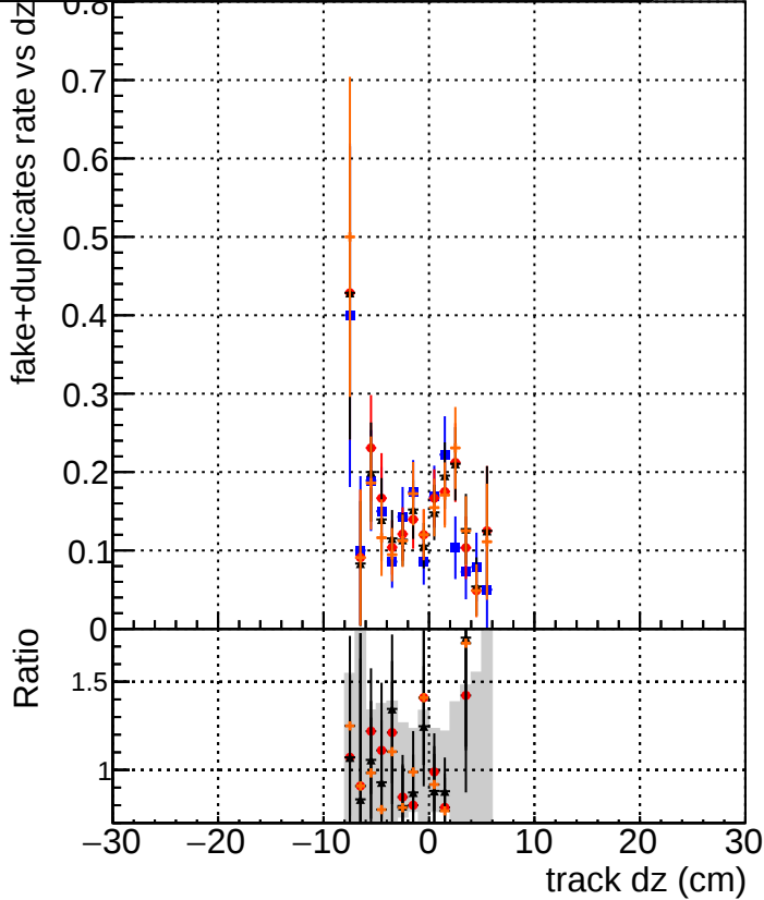
DQM_original4 DQM_testMkFit_initialStepReso DQM_testMkFitFit_initialStepReso DQM_testMkFitFit_initialStepReso_wRejection25
