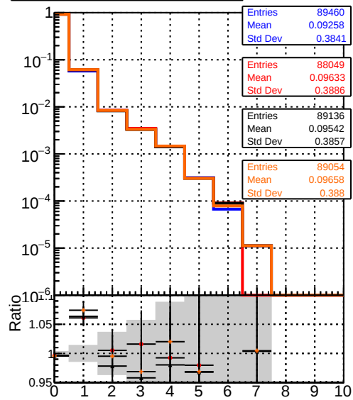
mean hit DQM_original4 DQM_testMkFit_initialStepReso DQM_testMkFitFit_initialStepReso DQM_testMkFitFit_initialStepReso_wRejection25
