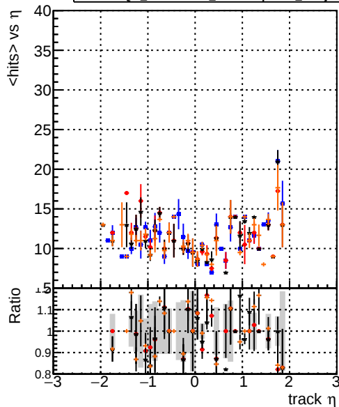
— DQM_testMkFit_initialStepReso — DQM_testMkFitFit_initialStepReso — DQM_testMkFitFit_initialStepReso_wRejection25 mean hit
