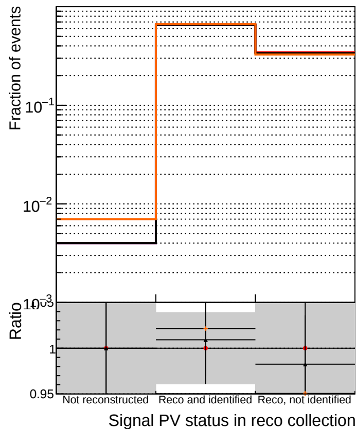
— DQM_original4 — DQM_testMkFit_initialStepReso — DQM_testMkFitFit_initialStepReso — DQM_testMkFitFit_initialStepReso_wRejection25
