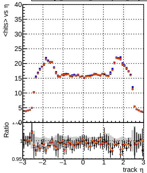
— DQM_original4 — DQM_testMkFit_initialStepReso — DQM_testMkFitFit_initialStepReso — DQM_testMkFitFit_initialStepReso_wRejection25 mean hit
