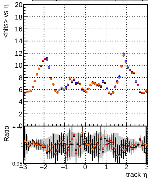
mean hits DQM_original4 DQM_testMkFit_initialStepReso DQM_testMkFitFit_initialStepReso DQM_testMkFitFit_initialStepReso_wRejection25
