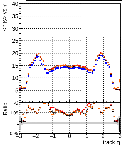
mean hit — DQM_origina14 — DQM_testMkFit_initialStepReso — DQM_testMkFitFit_initialStepReso — DQM_testMkFitFit_initialStepReso_wRejection25
