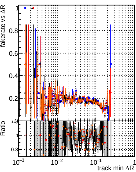
Fake rate vs \Delta R(\text{track, jet}) DQM original4 DQM testMKFit_initialStepReso DQM testMKFit_initialStepReso wRejection25
