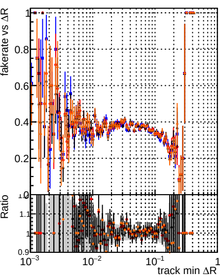
Fake rate vs \Delta R (track, jet) for various models and rejection methods.
