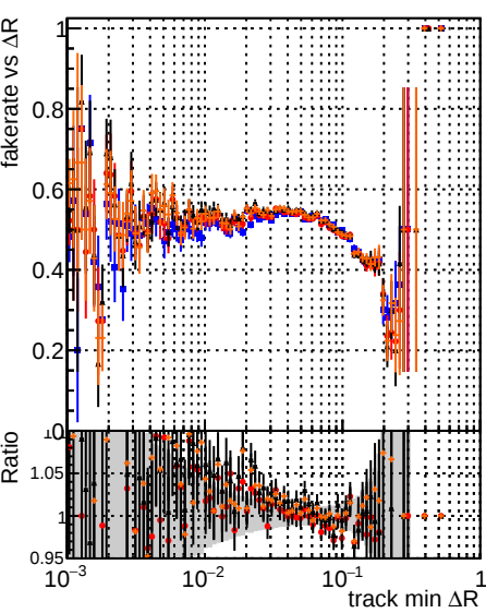
Legend: - \square original4 - \circ recoIMCFit_initialStepReso - \triangle recoIMCFit_initialStepReso_wRejection25 - \text{Ratio} (black line) - \text{Ratio} (shaded gray region)
