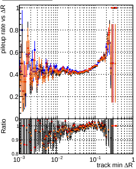
Legend: - \square original4 - \circ recoIMCFit_initialStepReso - \triangle recoIMCFit_initialStepReso_wRejection25 - \text{Ratio} (black line) - \text{Ratio} (shaded gray region)
