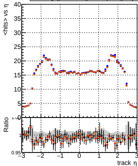
mean hit DQM_original14 DQM_testMkFit_initialStepReso DQM_testMkFitFit_initialStepReso DQM_testMkFitFit_initialStepReso_wRejection25
