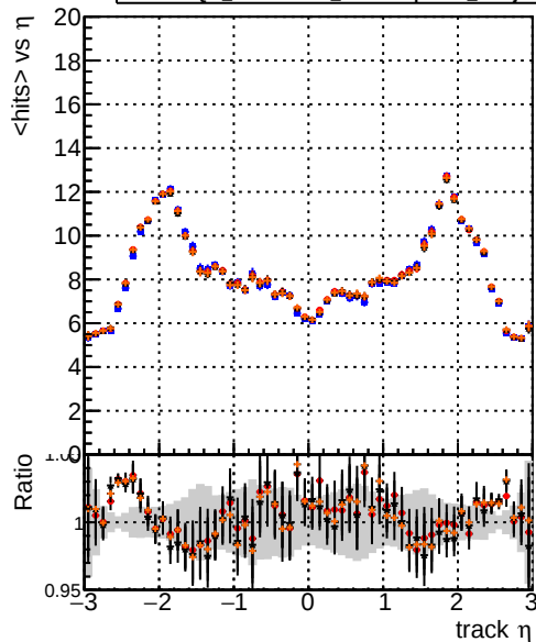
— DQM_original4 — DQM_testMkFit_initialStepReso — DQM_testMkFitFit_initialStepReso — DQM_testMkFitFit_initialStepReso_wRejection25 mean hits
