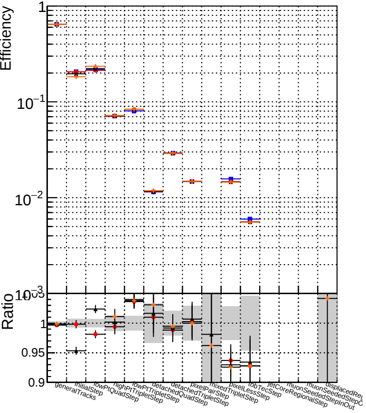
DQM_original4 DQM_testMkFit_initialStepReso DQM_testMkFitFit_initialStepReso DQM_testMkFitFit_initialStepReso_wRejection100
