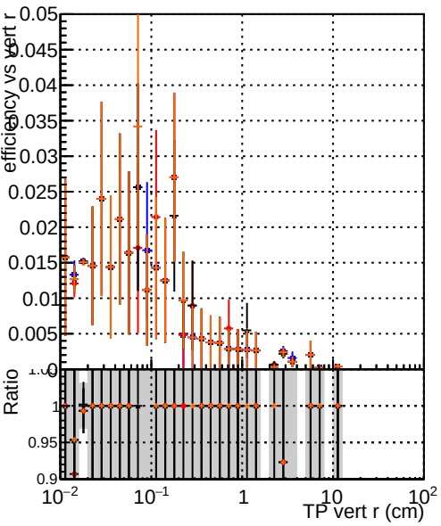
Efficiency vs TP vert r (cm) DOM_original4 DOM_testMkFit_initialStepReso DOM_testMkFitFit_initialStepReso DOM_testMkFitFit_initialStepReso_wRejection100
