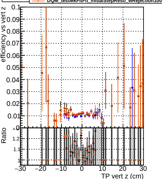
Efficiency vs vert z
