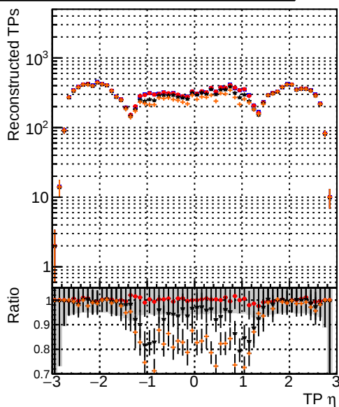
—●— DQM_original4 —●— DQM_testMkFit_initialStepReso —●— DQM_testMkFitFit_initialStepReso —●— DQM_testMkFitFit_initialStepReso_wRejection100
