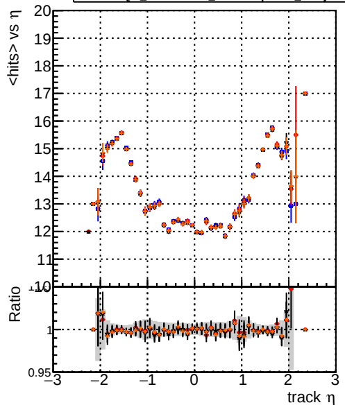
DQM_testMkFit_initialStepReso DQM_testMkFitFit_initialStepReso DQM_testMkFitFit_initialStepReso_wRejection100 mean hits
