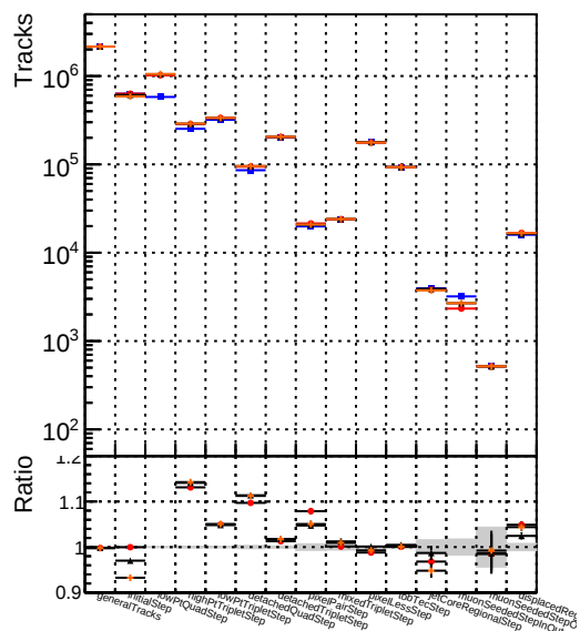
Number of tracks vs collection DQM_original4 DQM_testMkFitFit_initialStepReso DQM_testMkFitFit_initialStepReso DQM_testMkFitFit_initialStepReso_wRejection100
