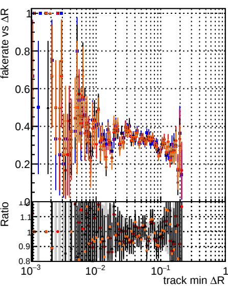
Fake rate vs \Delta R(\text{track, jet}) DQM original4 DQM testIMKFit_initialStepReso DQM testIMKFit_initialStepReso wRejection100
