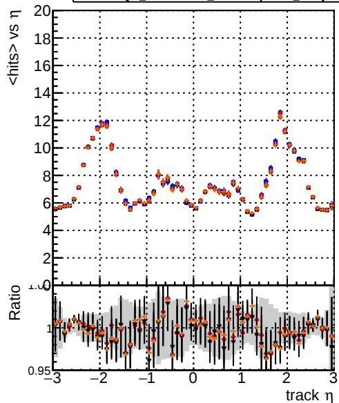
mean hits DQM_original4 DQM_testMkFit_fit_initialStepReso DQM_testMkFitFit_initialStepReso DQM_testMkFitFit_initialStepReso_wRejection100
