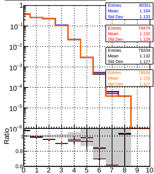
DQM_testMkFitFit_initialStepReso DQM_testMkFitFit_initialStepReso DQM_testMkFitFit_initialStepReso DQM_testMkFitFit_initialStepReso_wRejection100 mean hits
