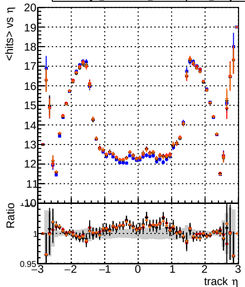
DQM_testMkFitFit_initialStepReso DQM_testMkFitFit_initialStepReso DQM_testMkFitFit_initialStepReso DQM_testMkFitFit_initialStepReso_wRejection100 mean hits
