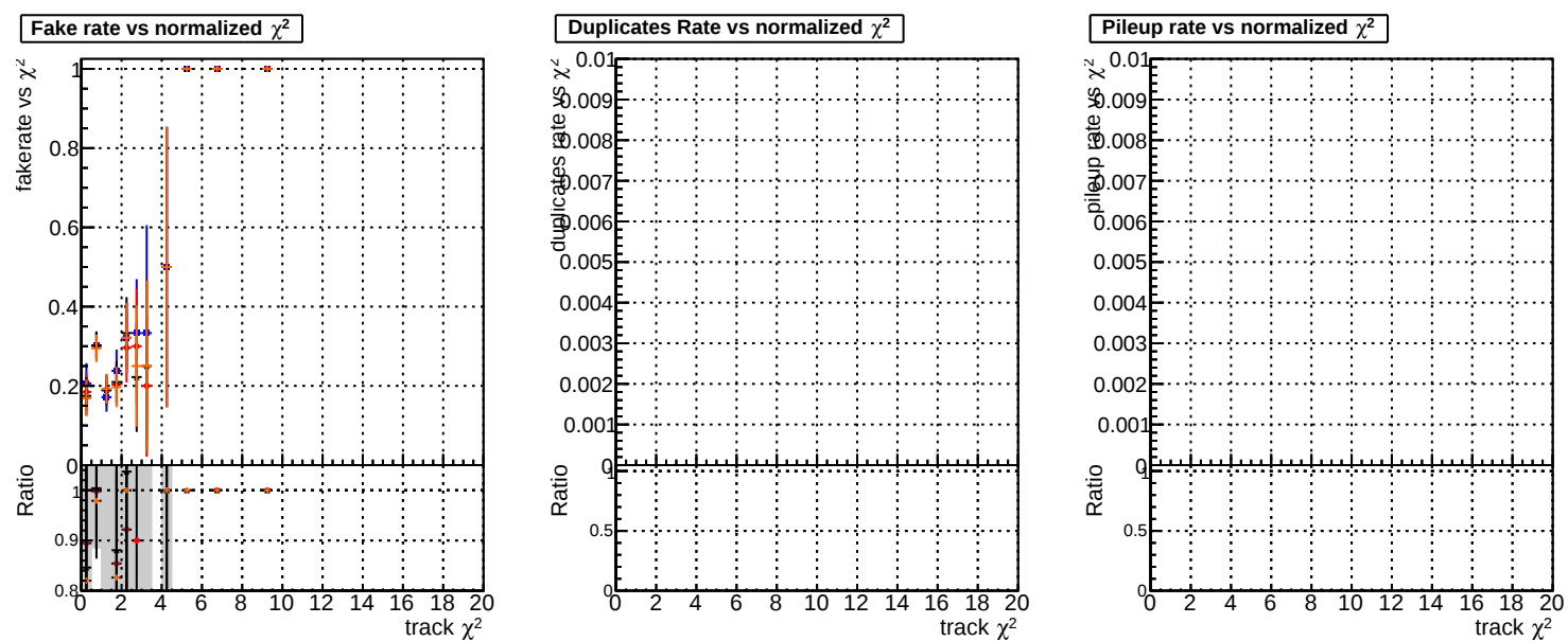
Fake rate vs. DOM original DOM test DOM test MKFit InitialStepReso DOM test MKFit InitialStepReso wRejection100
