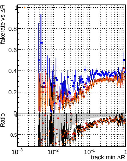
Fake rate vs \Delta R(\text{track, jet}) for various models and rejection levels.
