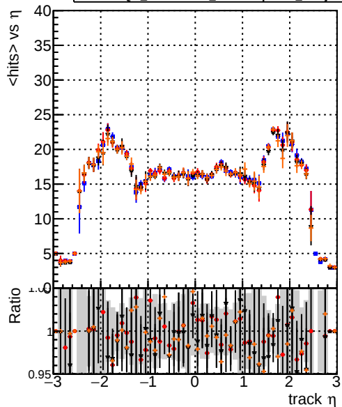
mean hit DQM_testMkFit_initialStepReso DQM_testMkFitFit_initialStepReso DQM_testMkFitFit_initialStepReso_wRejection100
