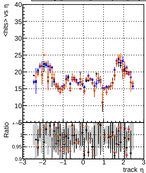
mean hits vs \eta Legend: Blue line: DQM_original4 Red line: DQM_testMkFit_initialStepReso Black line: DQM_testMkFitFit_initialStepReso Orange line: DQM_testMkFitFit_initialStepReso_wRejection100
